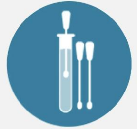
PCR test (polymerase chain reaction)
